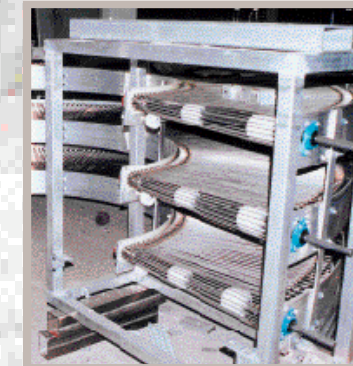
Multi-Tiered
